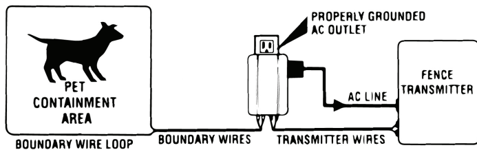
DRAWING 2
